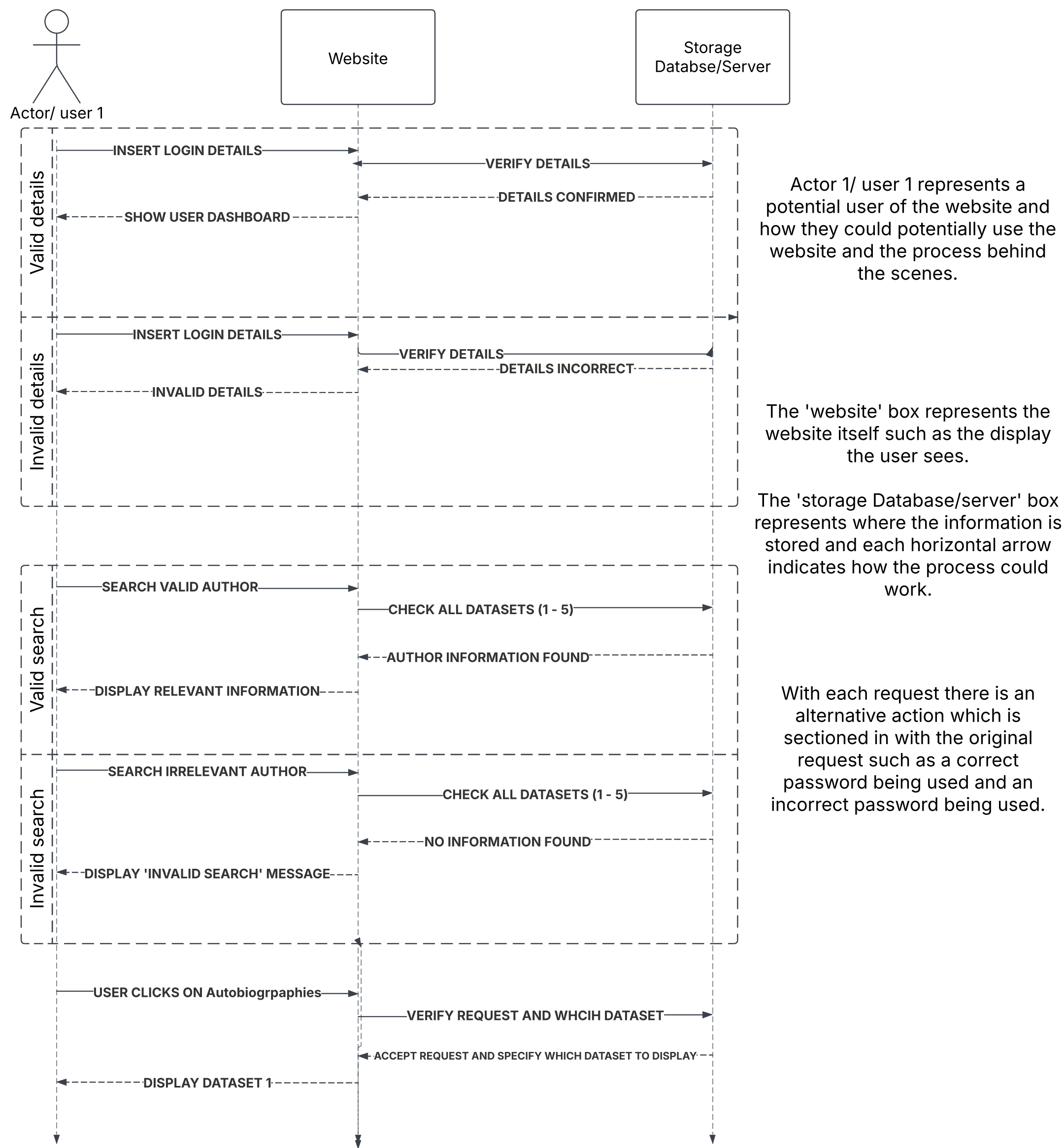
UML Sequence diagram
